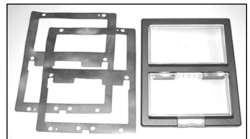
Bezel, Micro TK P/N 91-9303 Carrier P/N 20-91-9303
