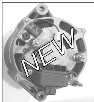
New 65 Amp Alternator TK P/N 41-5457 Carrier P/N 20-41-5457
