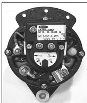
New 37 Amp Alternator TK P/N 41-2198 Carrier P/N 30-50337-00
