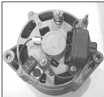
Reman 37Amp Alternator TK P/N 844-9571 Carrier P/N 20-44-9571RM
