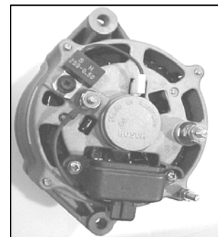
New 120 Amp Alternator TK P/N 41-5456 Carrier P/N 20-41-5456
