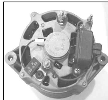
Reman 65 Amp Alternator TK P/N 844-9572 Carrier P/N 20-44-9572RM
