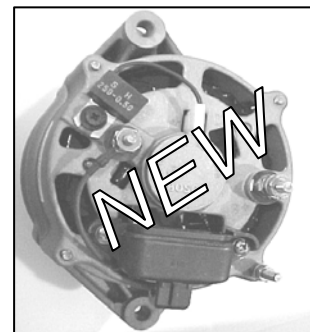
New 37 Amp Alternator TK P/N 41-5458 Carrier P/N 20-41-5458
