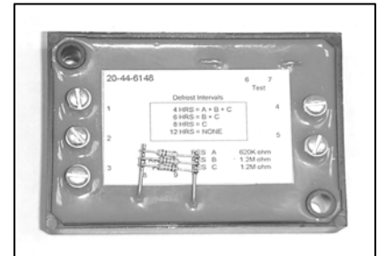
Defrost Timer TK P/N 44-6148 Carrier P/N 20-44-6148
