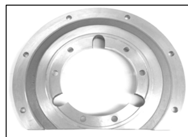
Flange, compressor TK P/N 22-723 Carrier P/N 20-22-723
