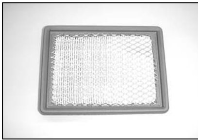
Air Filter (Truck Units) TK P/N 11-7234 Carrier P/N 20-11-7234
