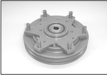
Centrifugal Clutch SB, Sentry, Super (50's) TK P/N 107-234 Carrier P/N 20-107-234
