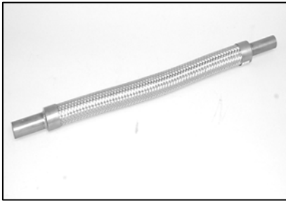
Discharge Vibe (SB III's & SB II Max) TK P/N 66-5784 Carrier P/N 20-66-5784
