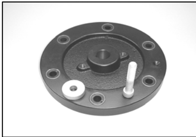
Coupling, 6 Pin (2.2DI & Std. Shaft X430) TK P/N 77-2504 Carrier P/N 20-77-2504
