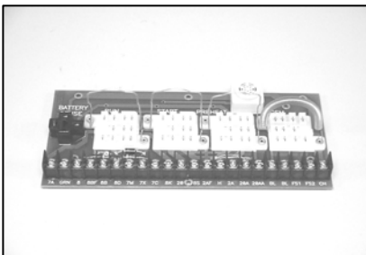
Board (P.C. CS-II w/buzzer) TK P/N 44-7246 Carrier P/N 20-44-7246
