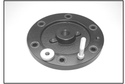
Coupling (2.2DI & Large Shaft X430) TK P/N 77-2509 Carrier P/N 20-77-2509
