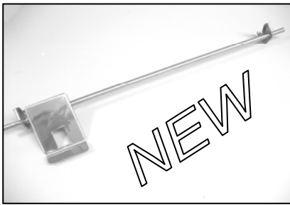
Latch, Door TK P/N 91-9621 Carrier P/N 20-91-9621
