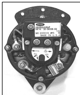
New 65 Amp Alternator TK P/N 41-2200 Carrier P/N 30-50336-00
